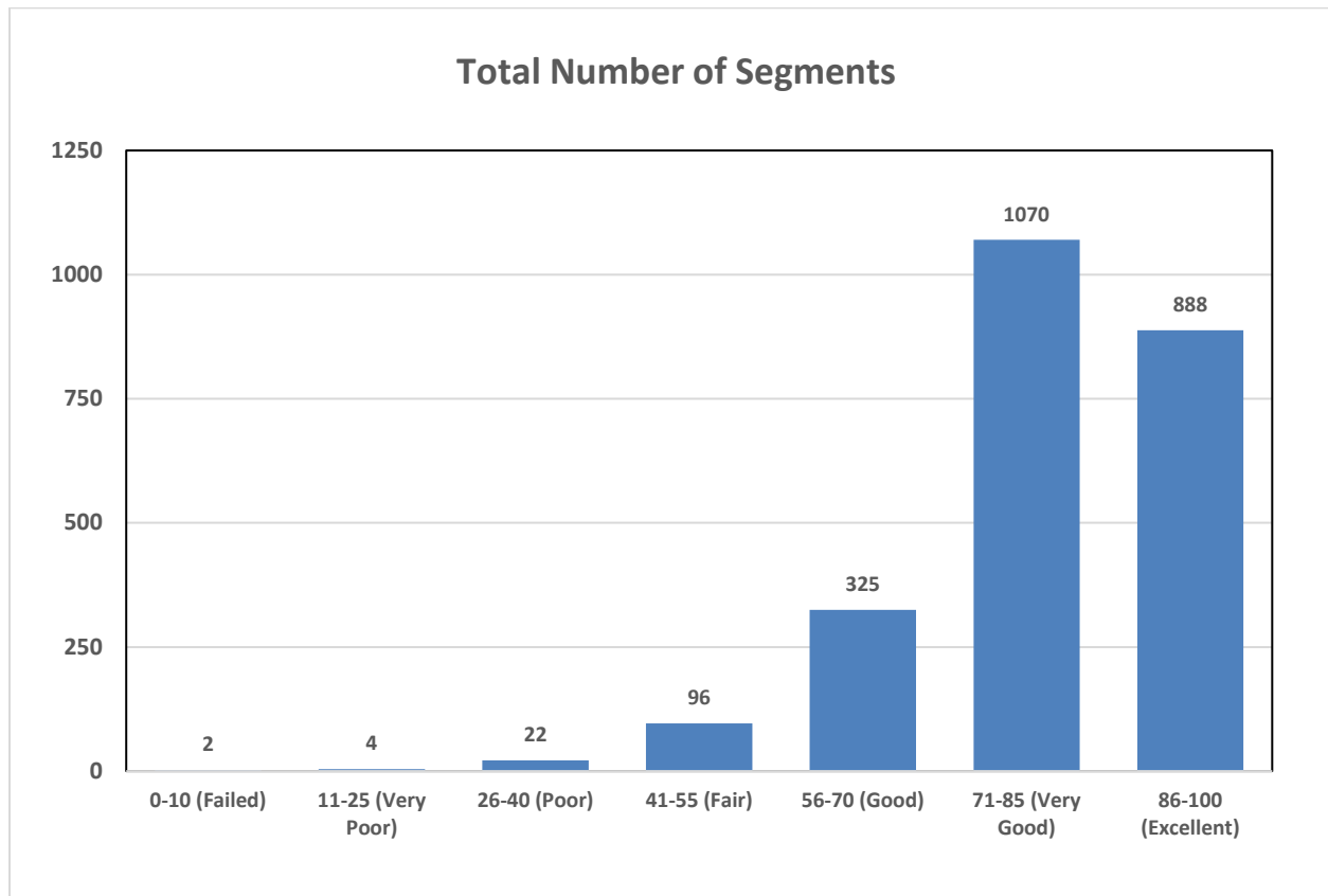
Figure 1 – 2022 Pavement Condition Results, Total Number of Segments
