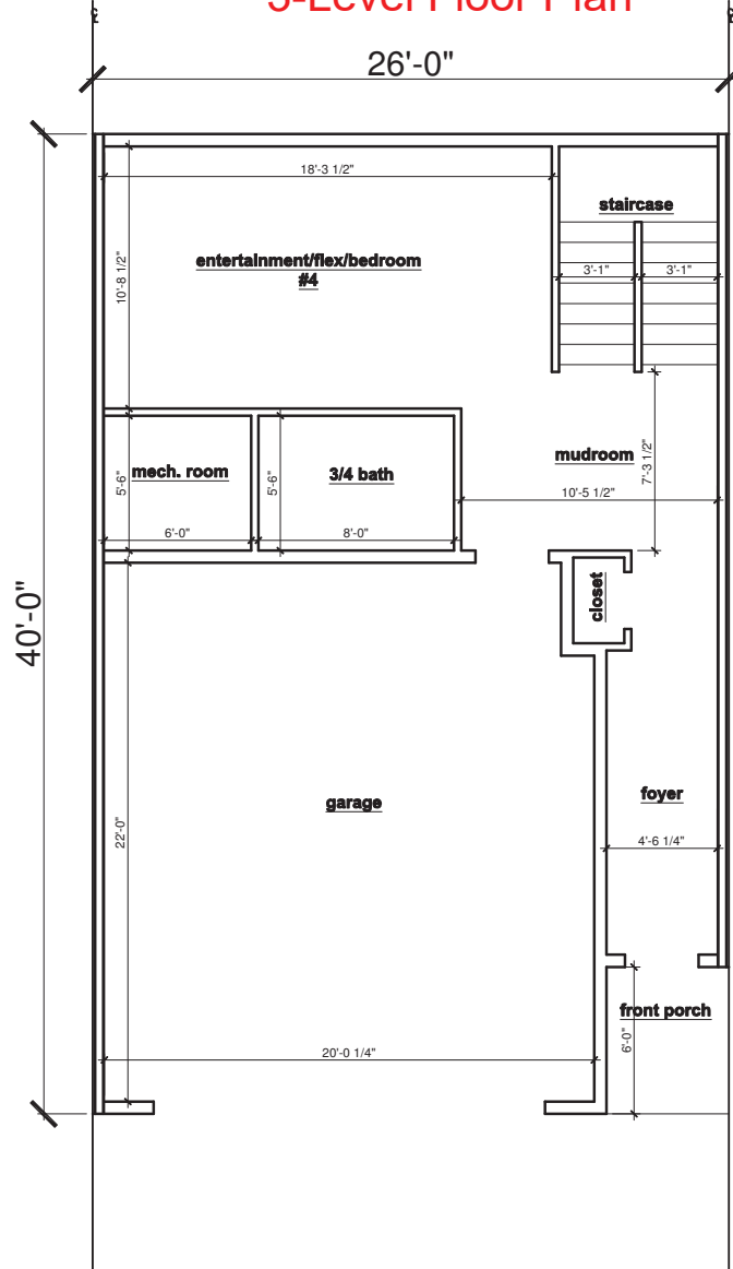
1 PROPOSED LOWER LEVEL 512 FINISHED SQUARE FEET / 40 MECH. ROOM SQUARE FEET / 459 GARAGE SQUARE FEET
