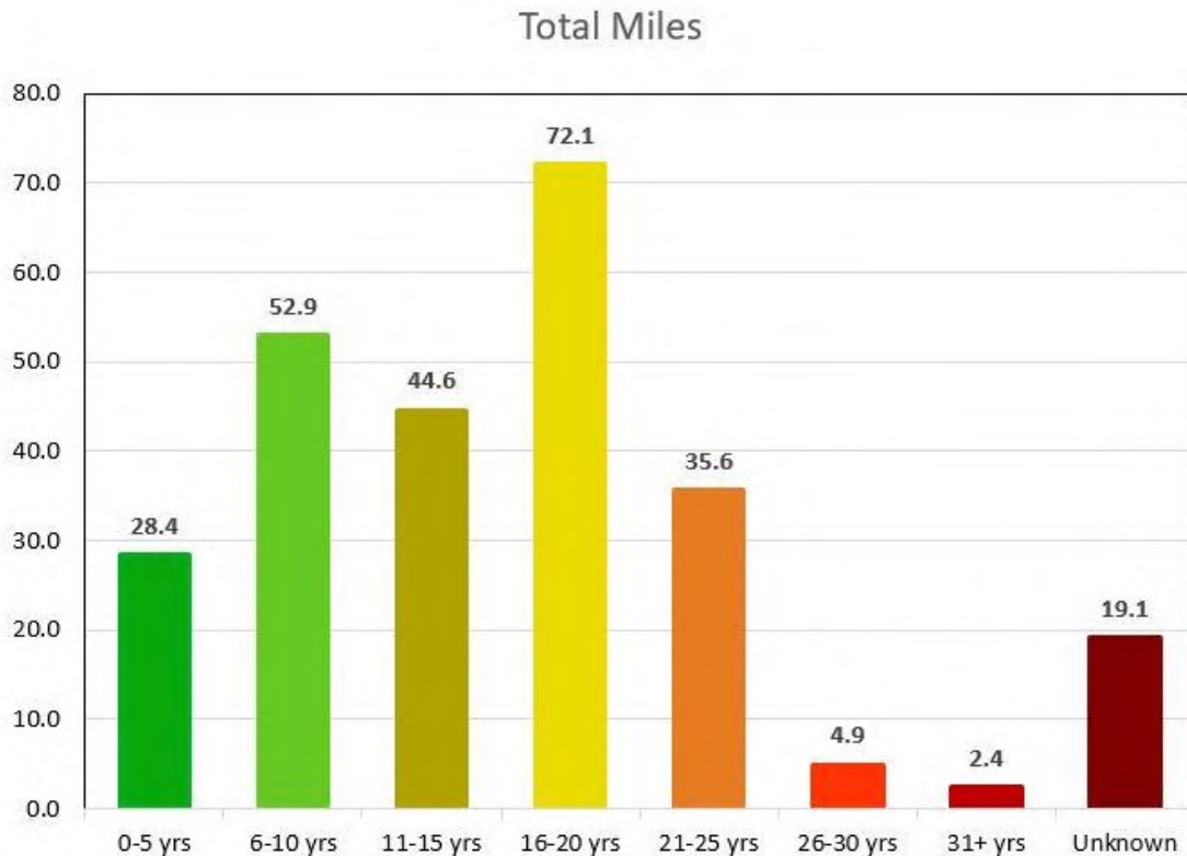
Figure 6: Pavement Age
