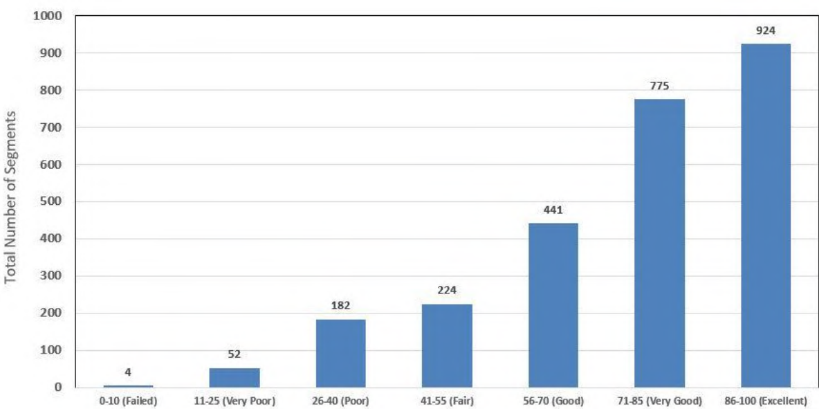
Figure 1 – Pavement Condition Results, Total Number of Segments
