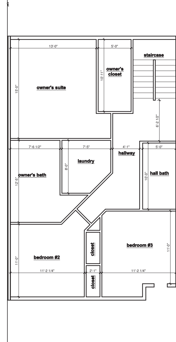
3 PROPOSED UPPER LEVEL 1030 FINISHED SQUARE FEET
