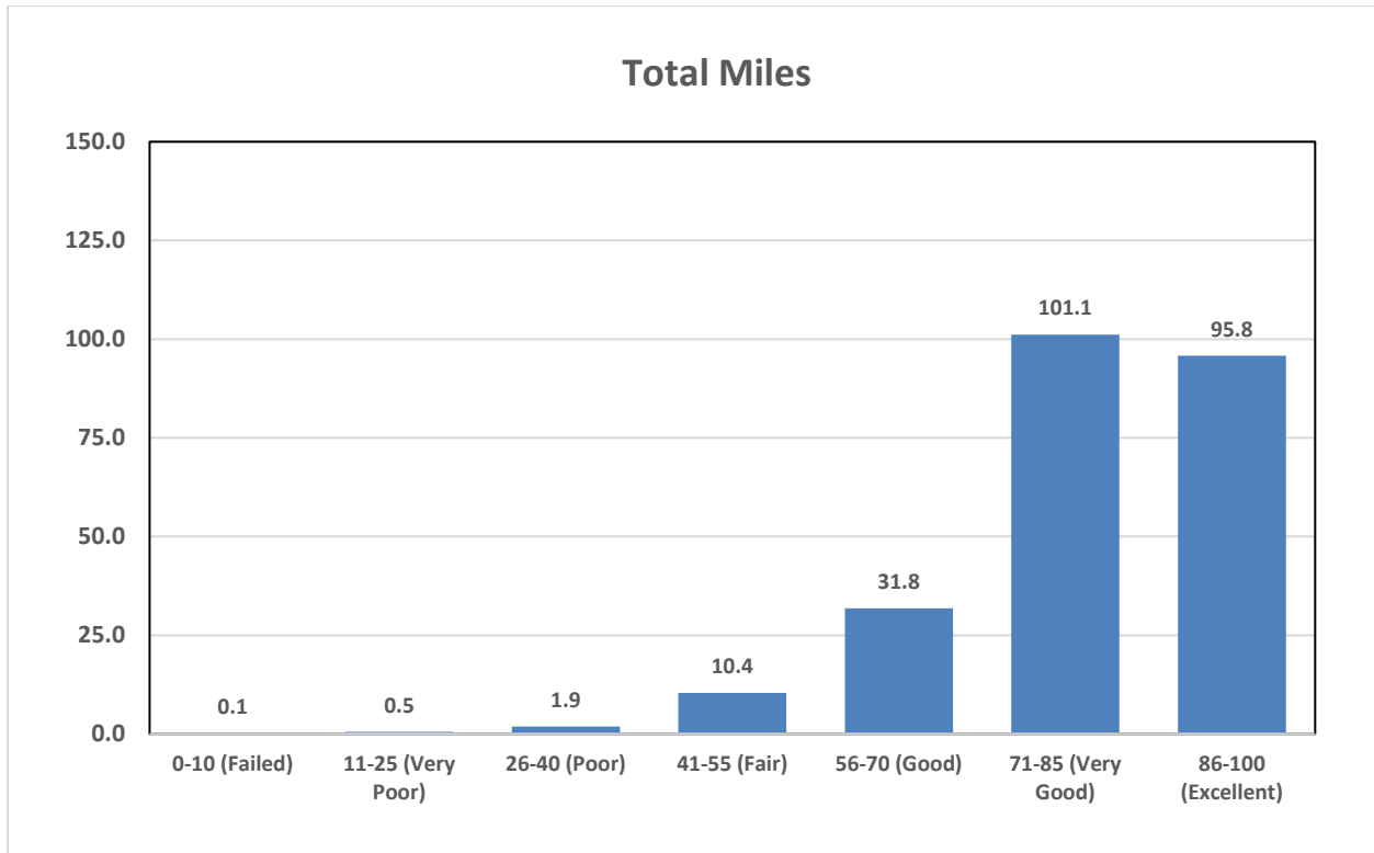
Figure 2 – 2022 Pavement Condition Results, Total Miles
