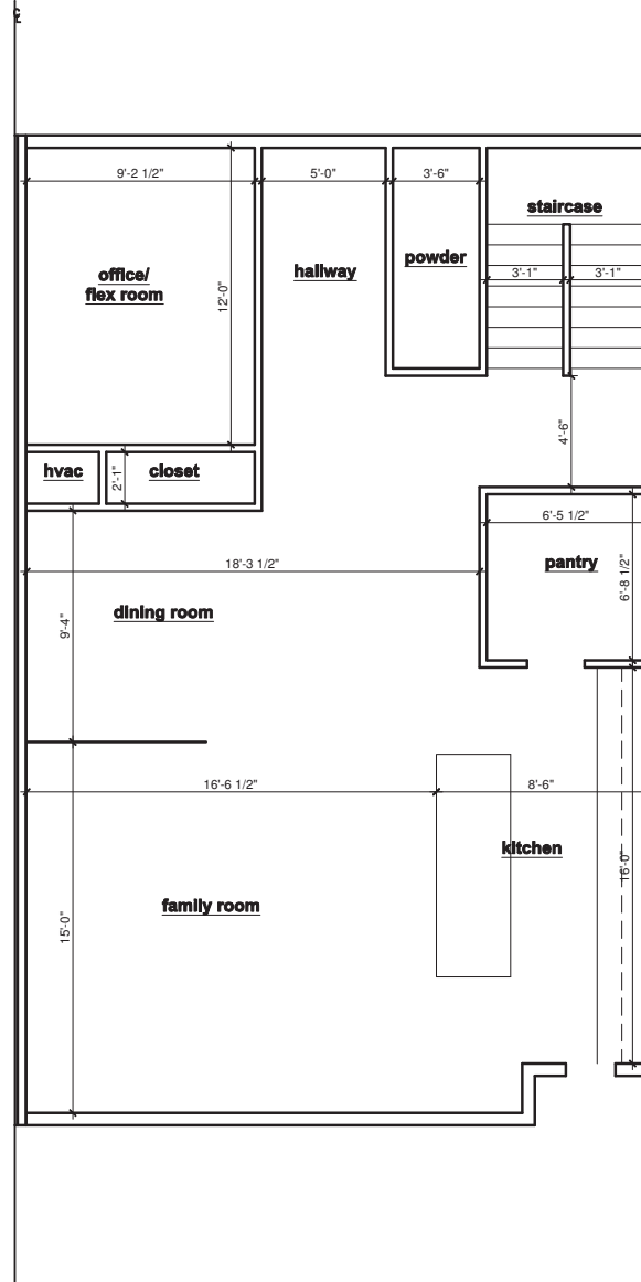
2 PROPOSED MAIN LEVEL 965 FINISHED SQUARE FEET
